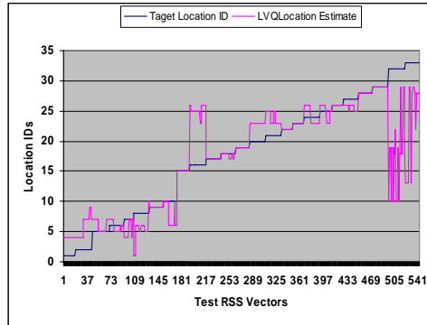
Figure 14: LVQ Performance on Testing Radio Map
